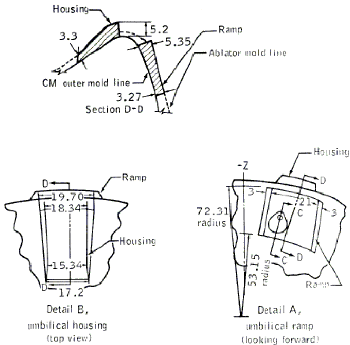
(e) Details of umbilical system.
