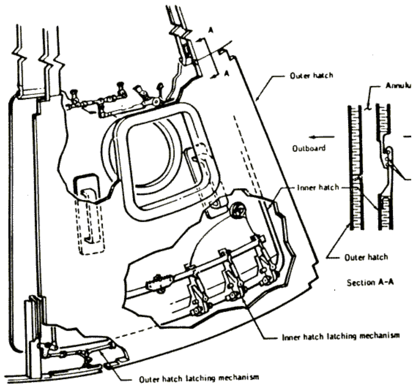
Figure 4-10.- Original side access hatch mechanism.
