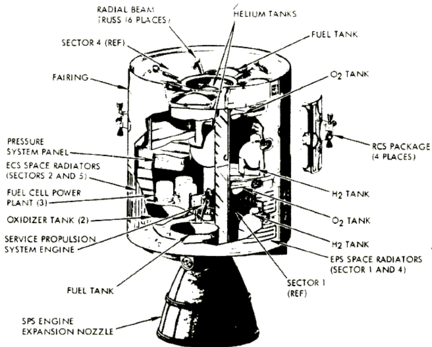
Service module (Block I)
