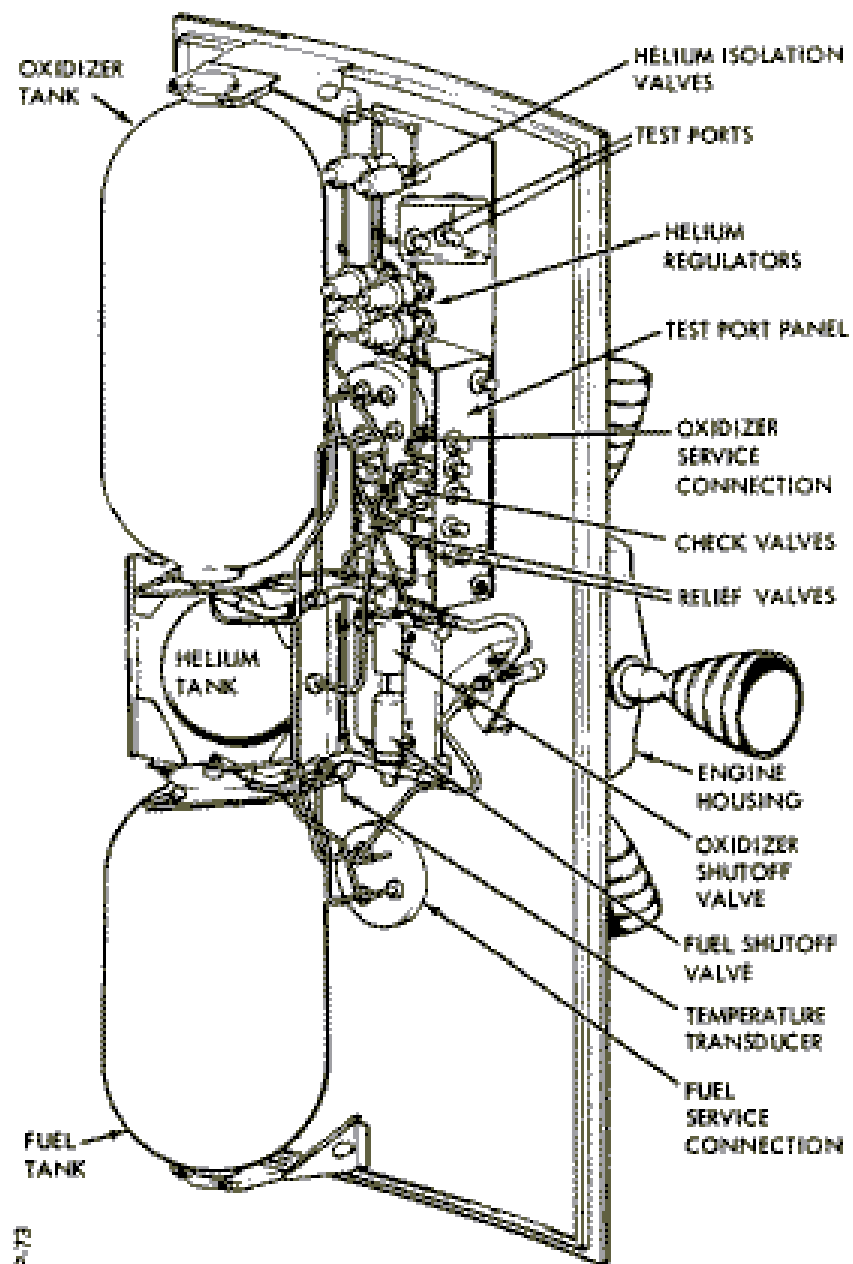
SM RCS quad assembly (Block I)
