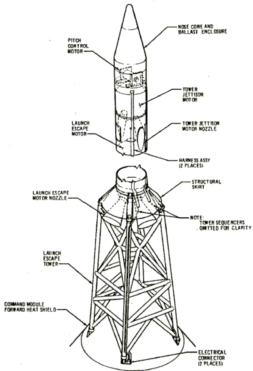
FIGURE V-2. LAUNCH ESCAPE SYSTEM
