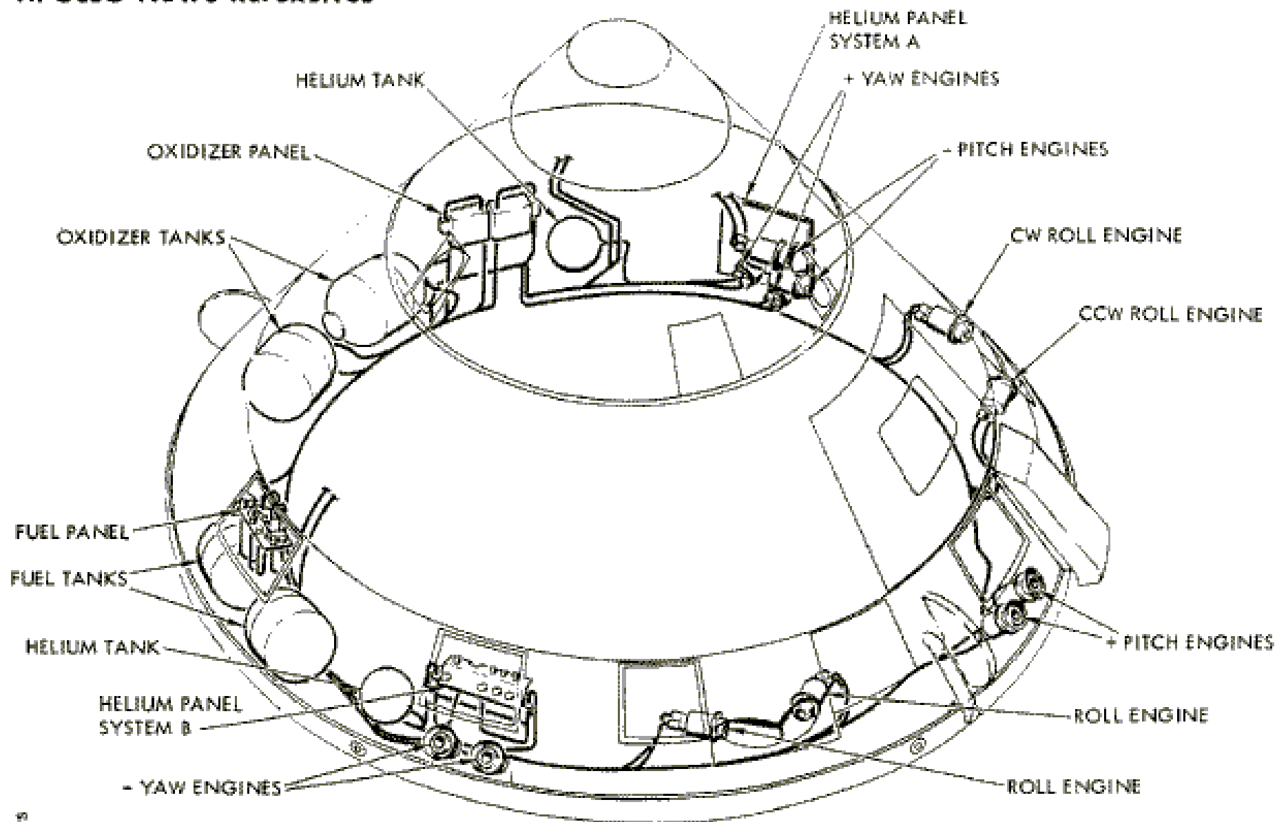
RCS component location on command module
