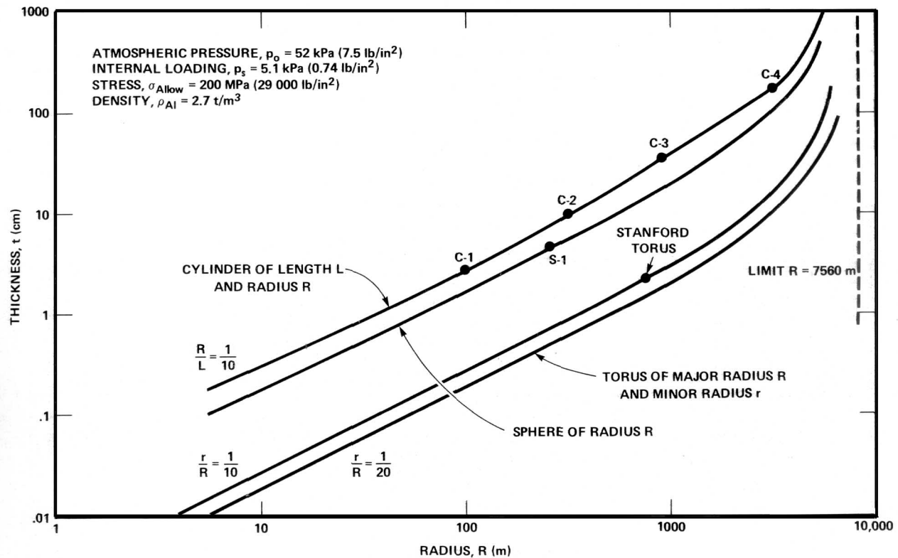
Figure 4-3 — Shelf thickness as a function of radius for spheres, cylinders, and toruses spinning to produce 1 g.
