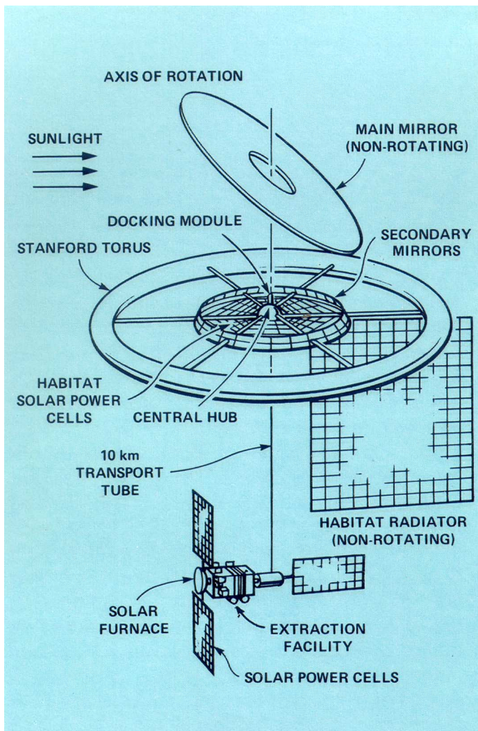
Figure 5-1 — Colony configuration.
