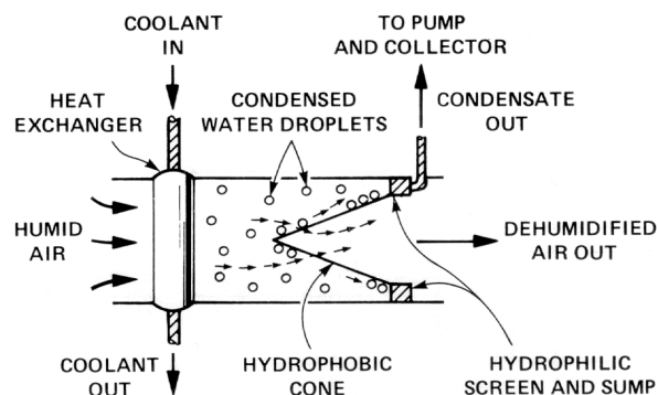
Figure 5-13 — Water removal.
