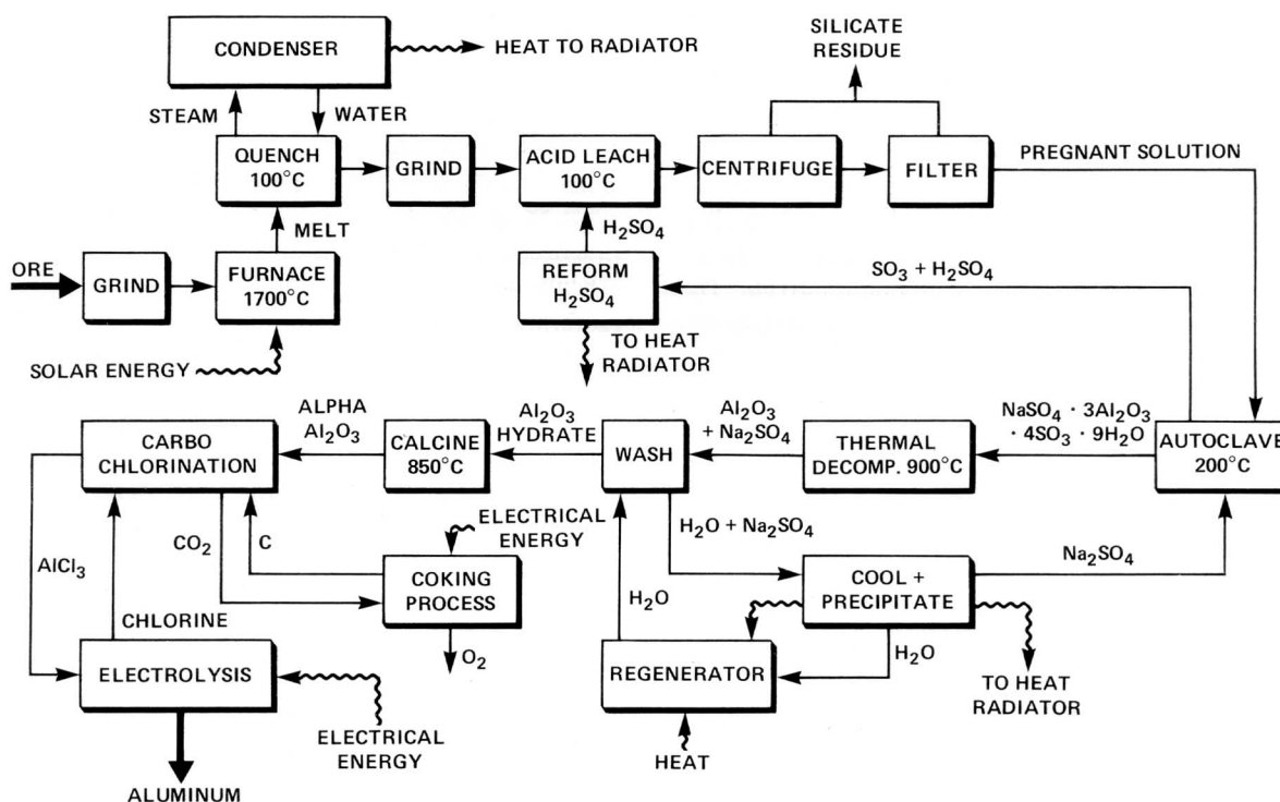
Figure 4-25 — Aluminum processing.
