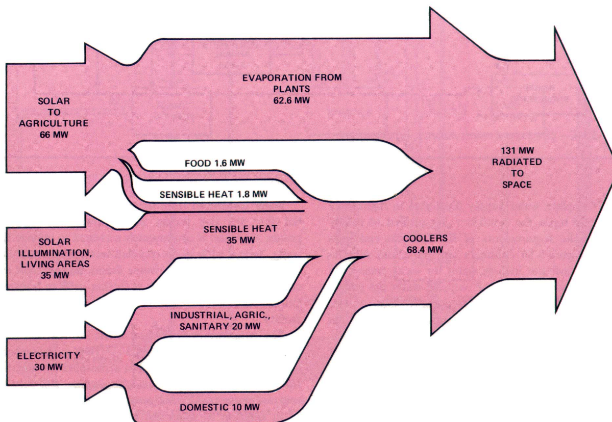
Figure 5-18 — Energy flow in the colony.
