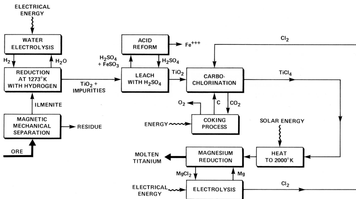
Figure 4-24 — Titanium processing.
